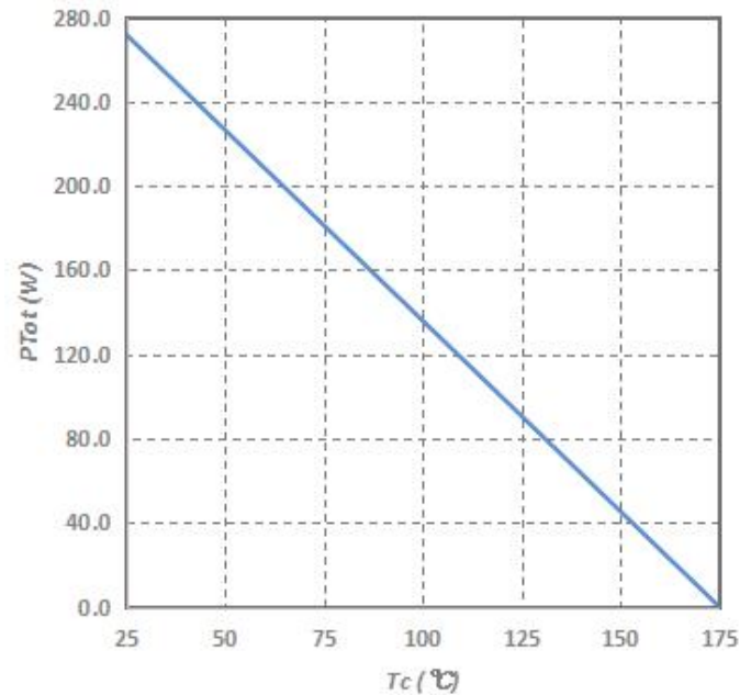
Fig.6-Power Derating
