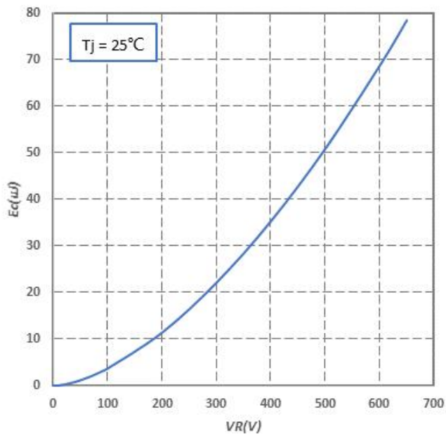
Fig.5-Capacitance Stored Energy
