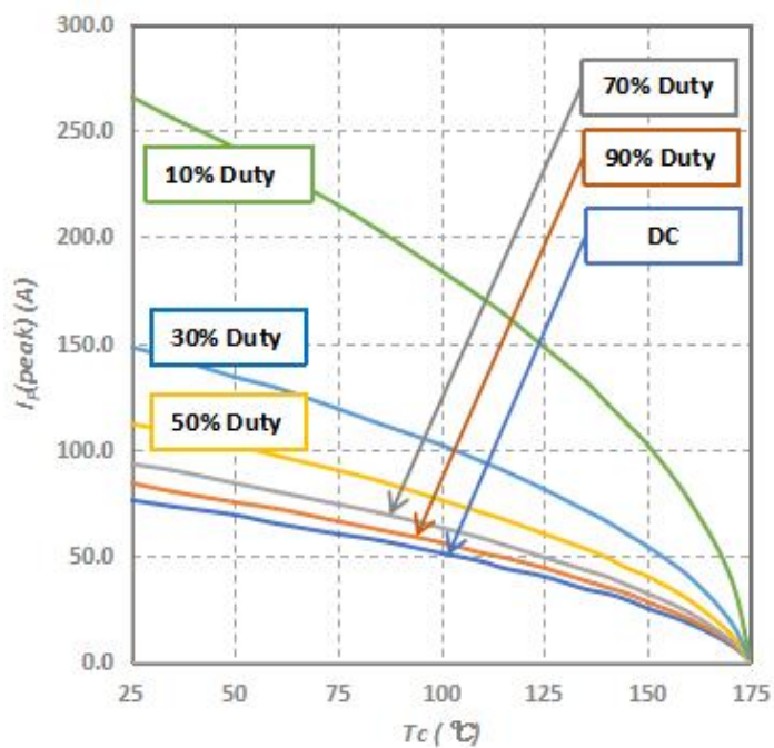
Fig.7-Current Derating
